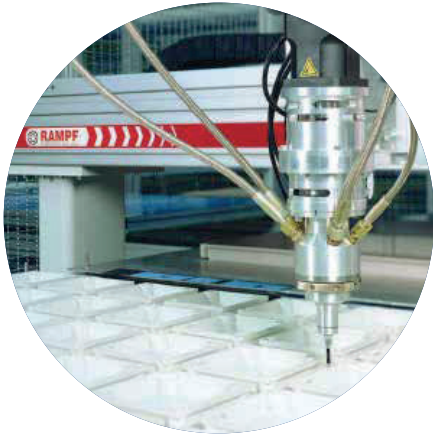
Automated gasket filling technology (FIPFG)*
